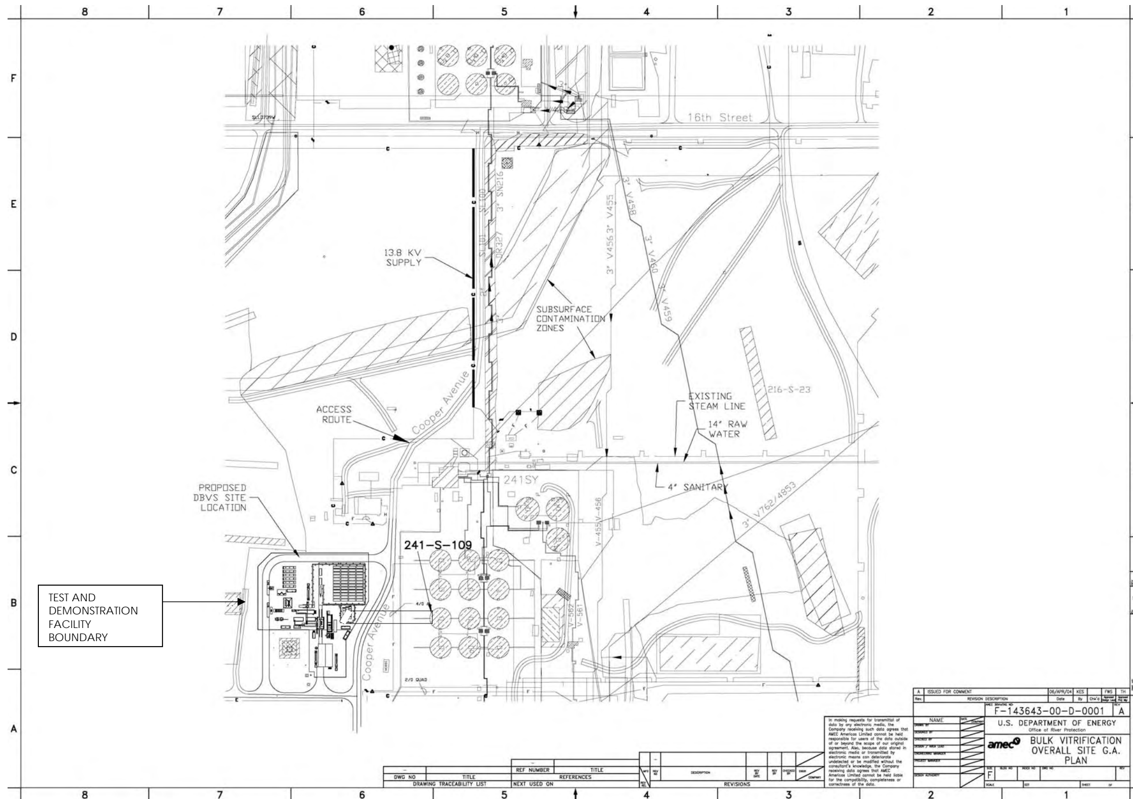
Figure 2-1. Planned Site Location of the Test and Demonstration Facility OFFICIAL USE ONLY
