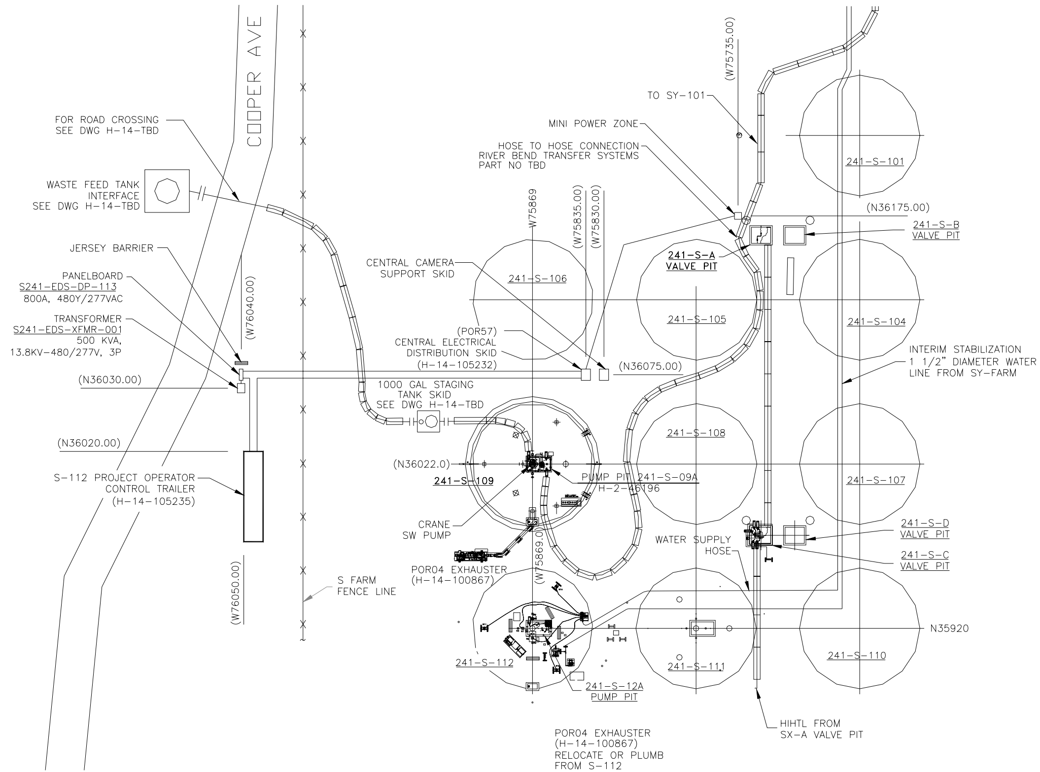
Figure 2-3. Test and Demonstration Facility Site and Equipment Layout - Page 2
