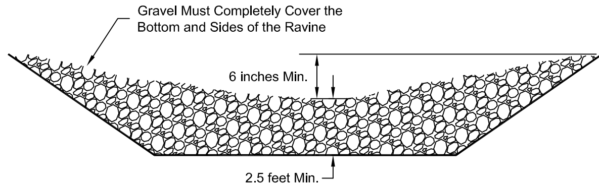
SECTION ACROSS RAVINE CENTERLINE
