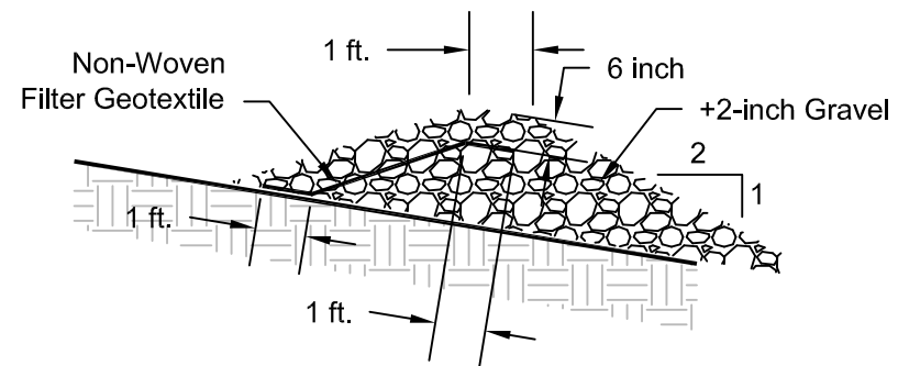
PROFILE ALONG RAVINE CENTERLINE
