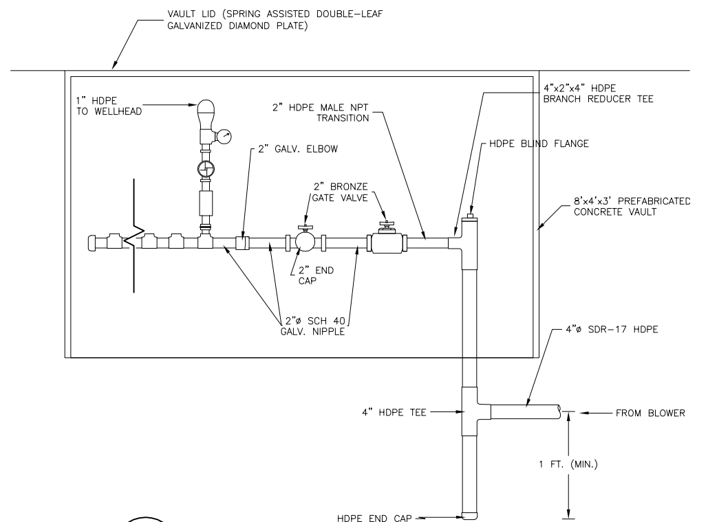
4 VAULT/MANIFOLD DETAIL C-20 SCALE: NTS
