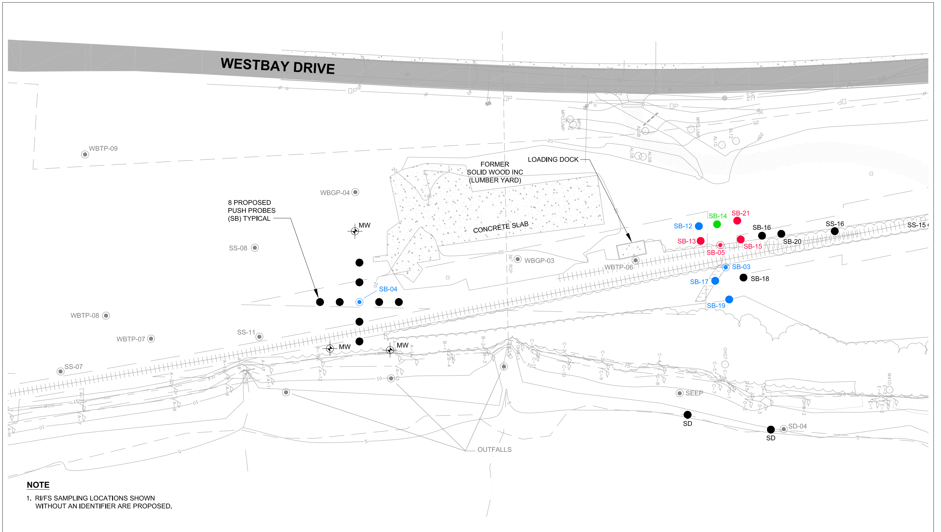
Figure 4 Solid Wood Incorporated Site (West Bay Park) Olympia, Washington Phase II ESA and RI/FS Sample Locations Central Site Area
