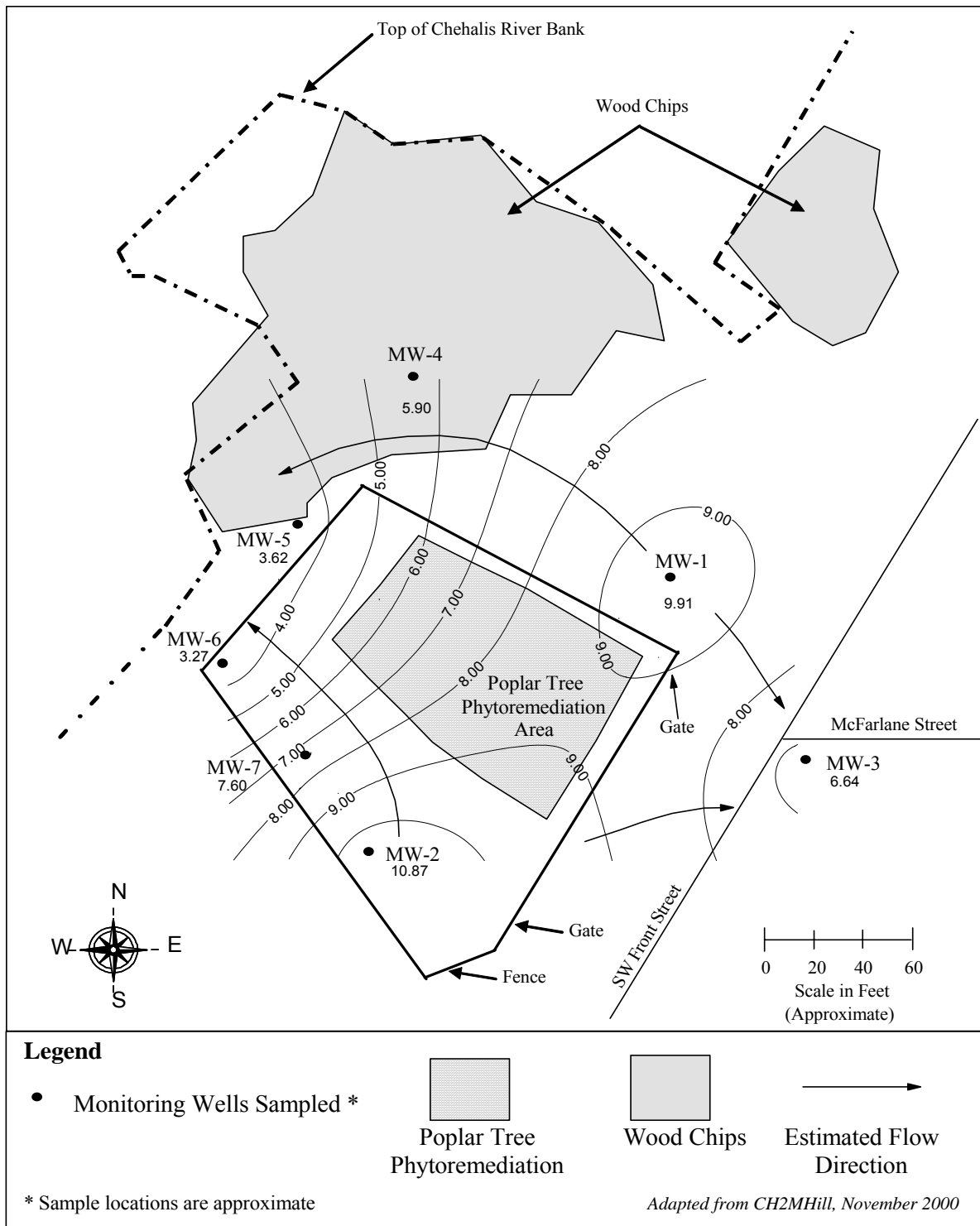
Figure 4: Saginaw Mill Groundwater Contour Map - April 2006
